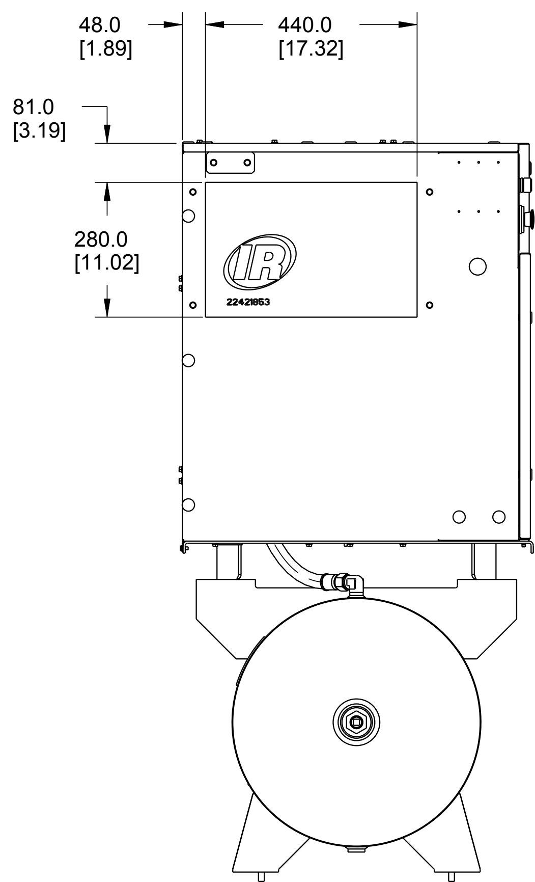
LEFT VIEW WITHOUT ODM ENCLOSURE
