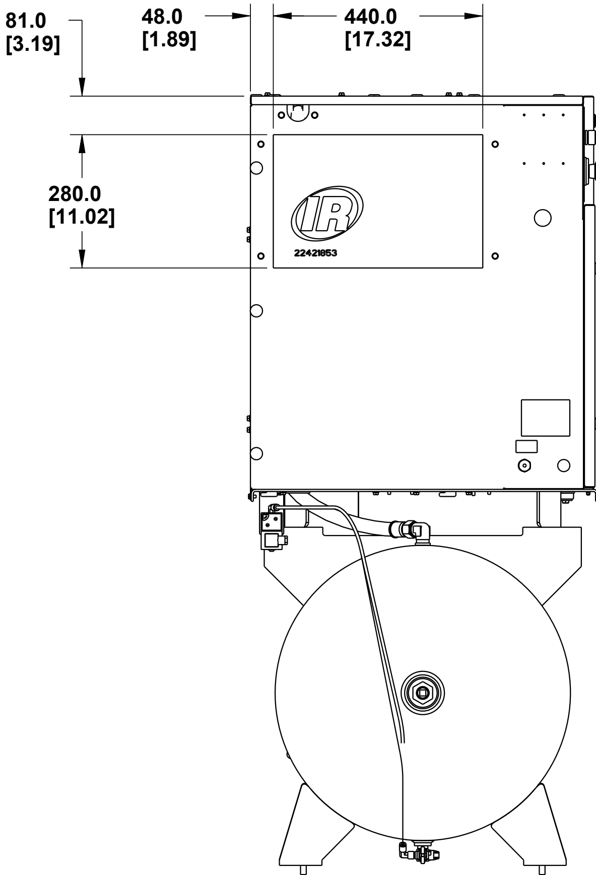
LEFT VIEW WITHOUT ODM ENCLOSURE
