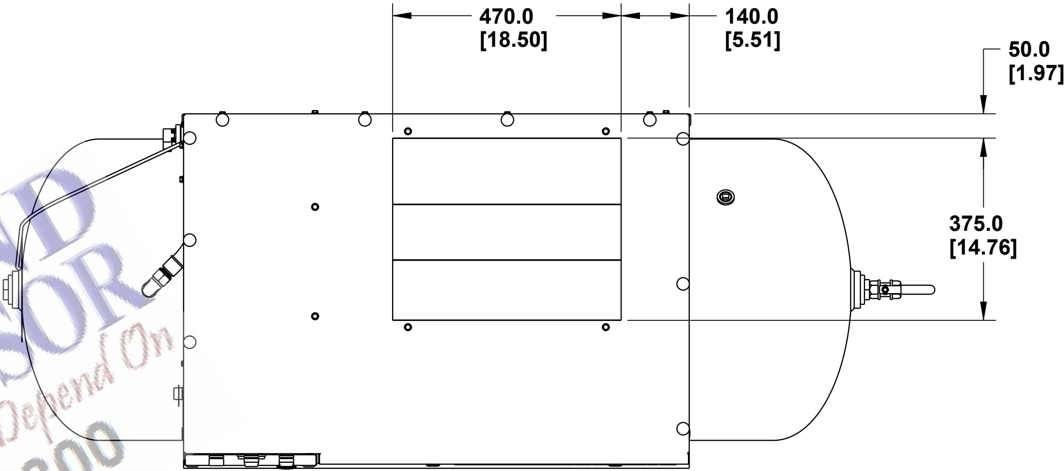
TOP VIEW WITHOUT ODM ENCLOSURE
