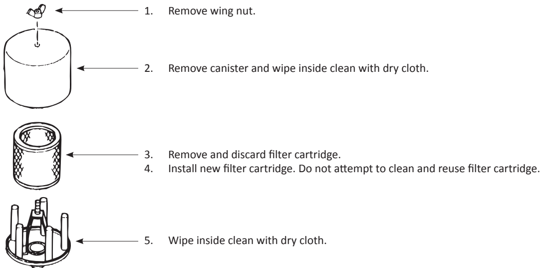
Figure 5 - Air Filter Replacement
